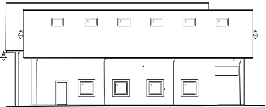
EXISTING ELEVATION 4
