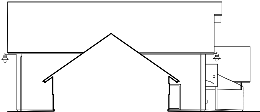
EXISTING ELEVATION 6
