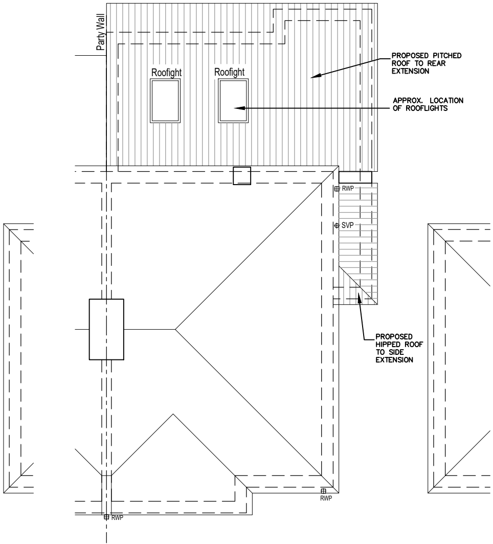
ROOF PLAN
