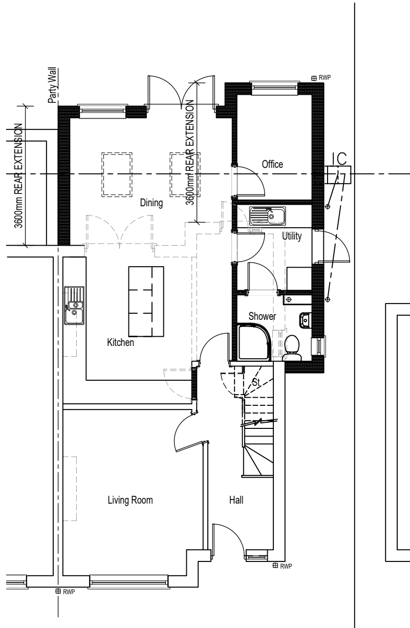
6 DEVON WAY GROUND FLOOR PLAN
