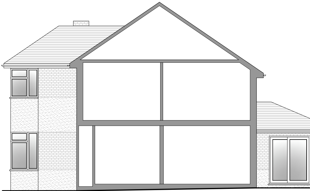
9 Existing Side Section
