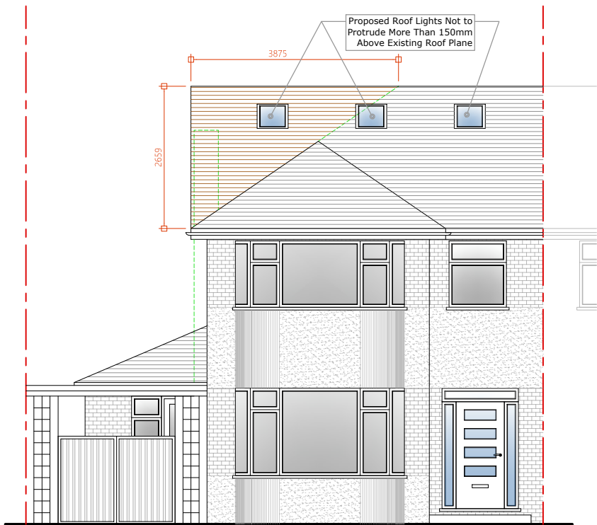
4 Proposed Front Elevation
