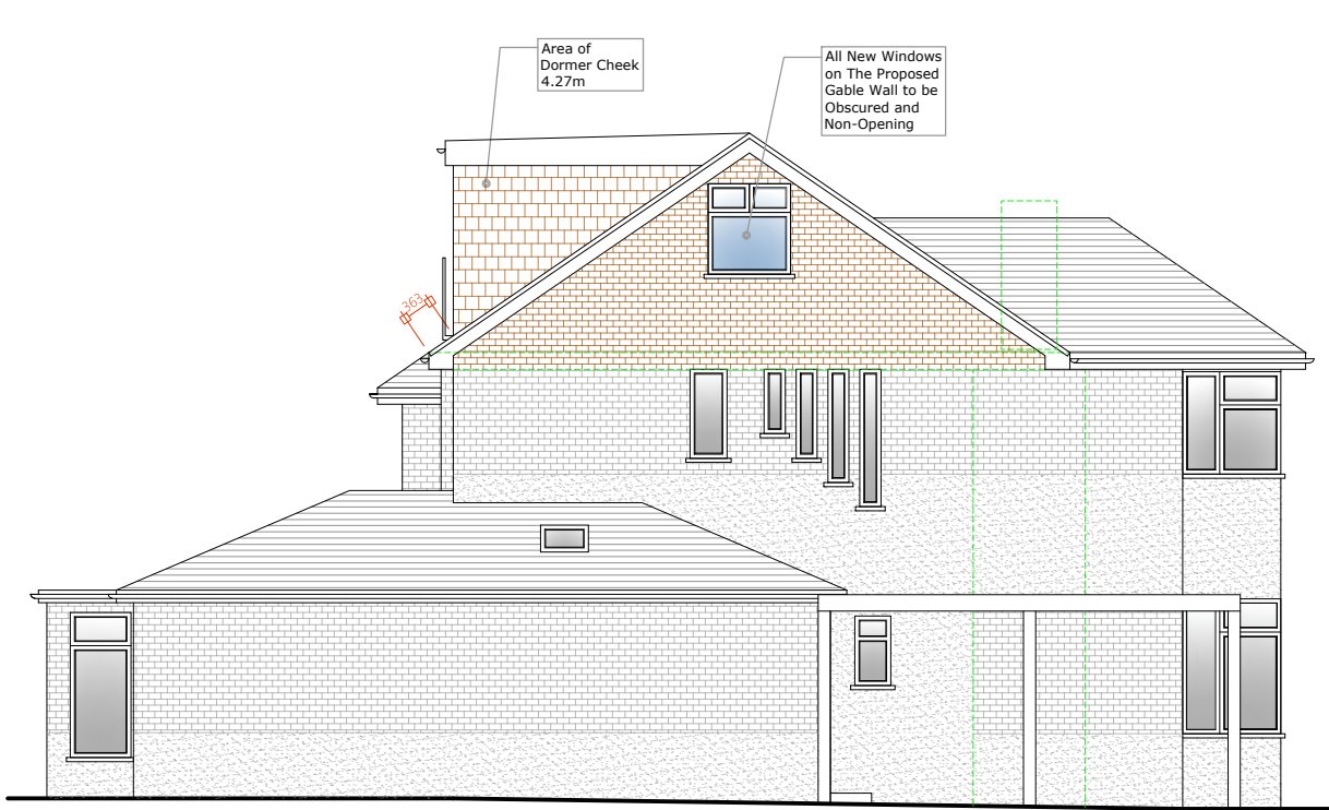
5 Proposed Side Elevation
