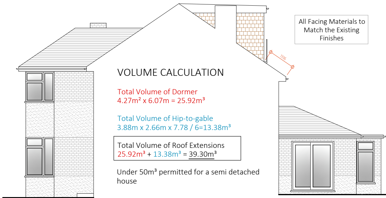
7 Proposed Side Elevation
