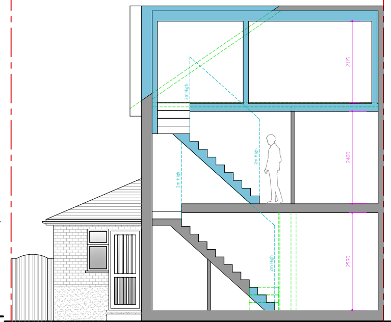
8 Proposed Front Section
