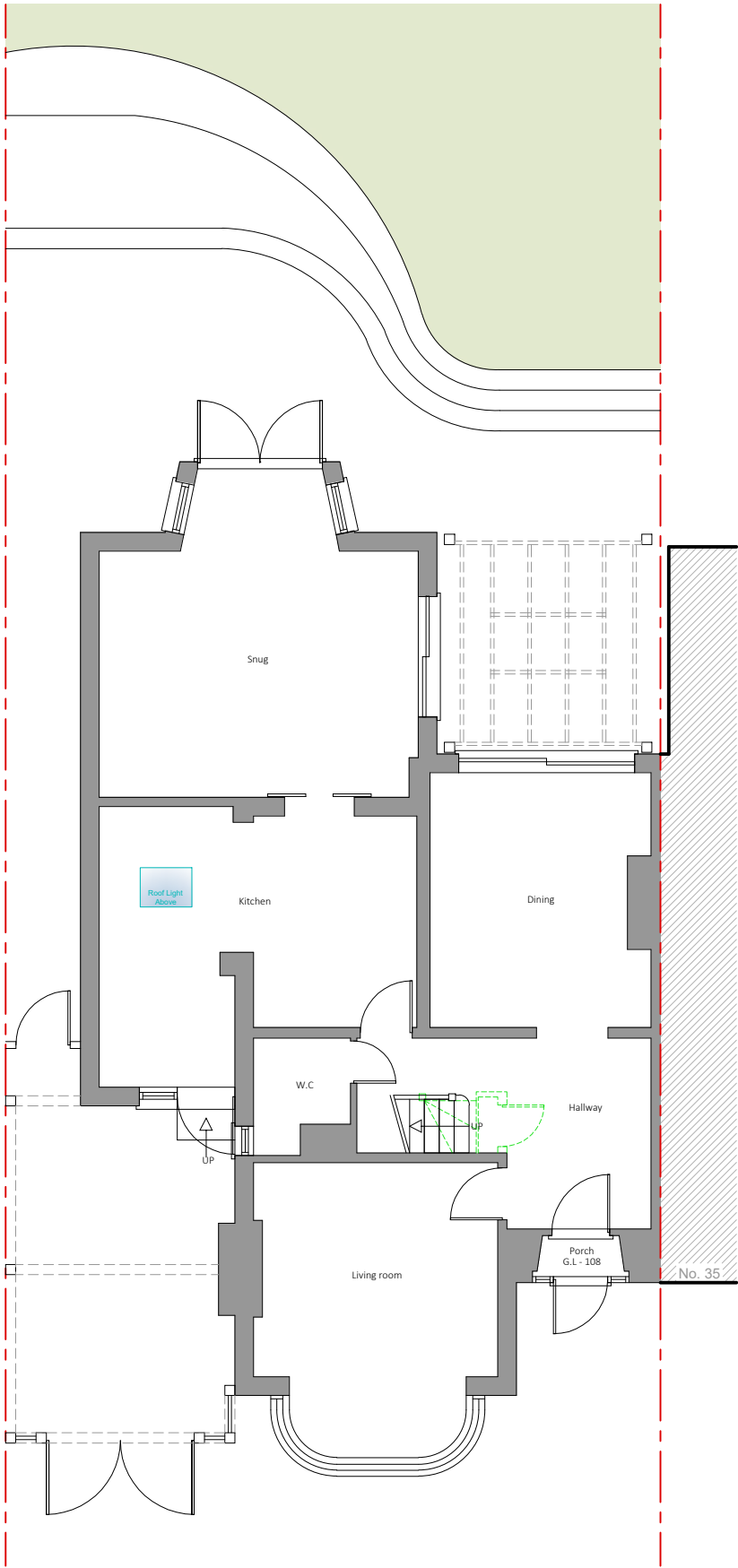
1 Proposed Ground Floor Plan
