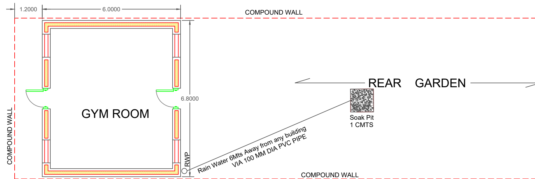
PROPOSED OUT BUILDING (AS GYM ROOM)
