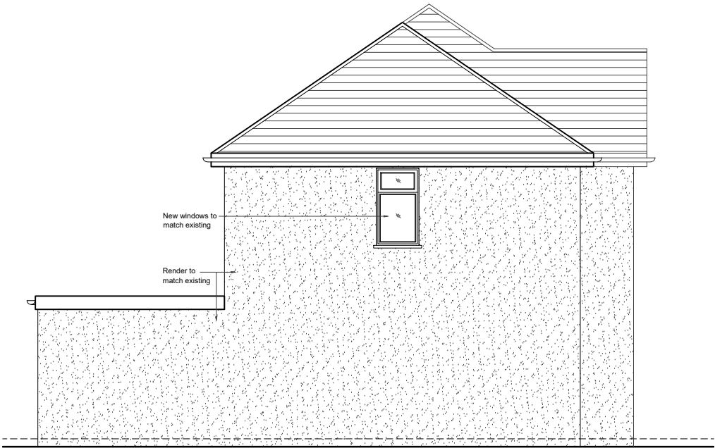
02 - SIDE ELEVATION
