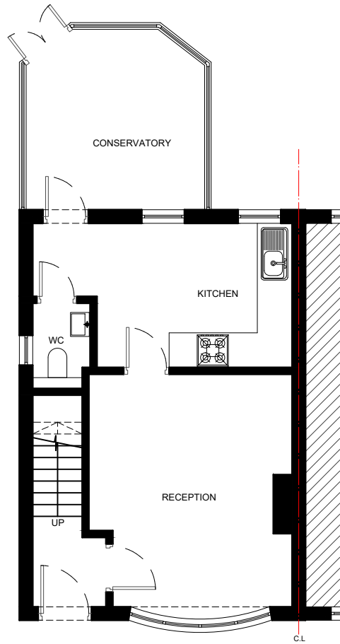
01 -GROUND FLOOR PLAN
