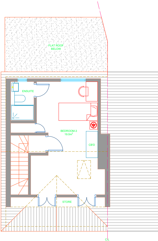
03 - LOFT FLOOR PLAN
