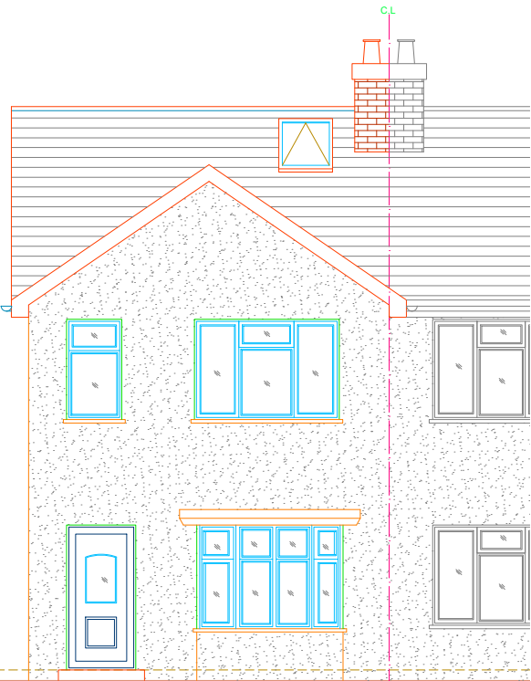
05 - FRONT ELEVATION
