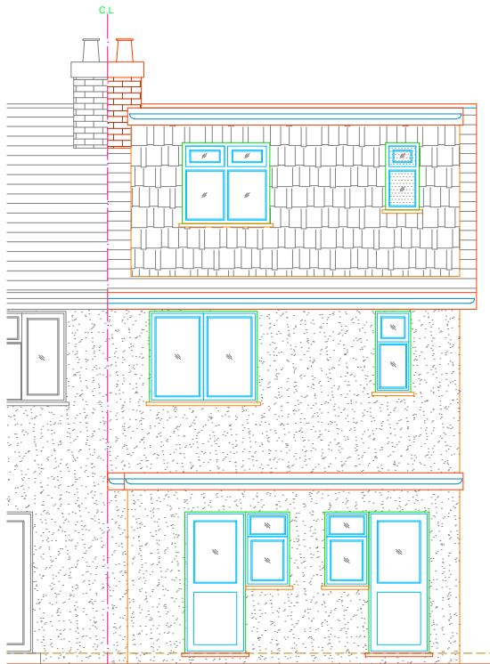
06 - REAR ELEVATION
