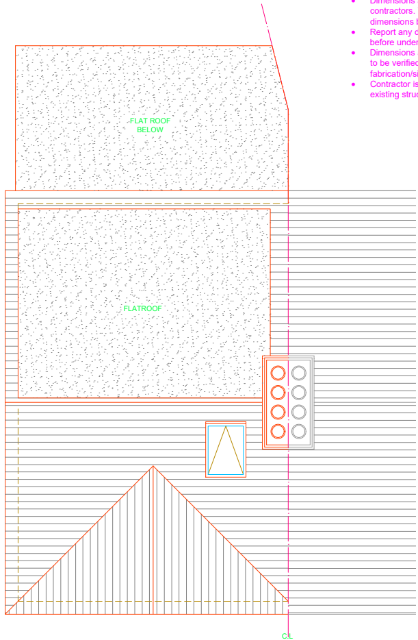
04 - ROOF PLAN
