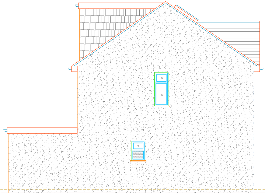
07 - SIDE ELEVATION
