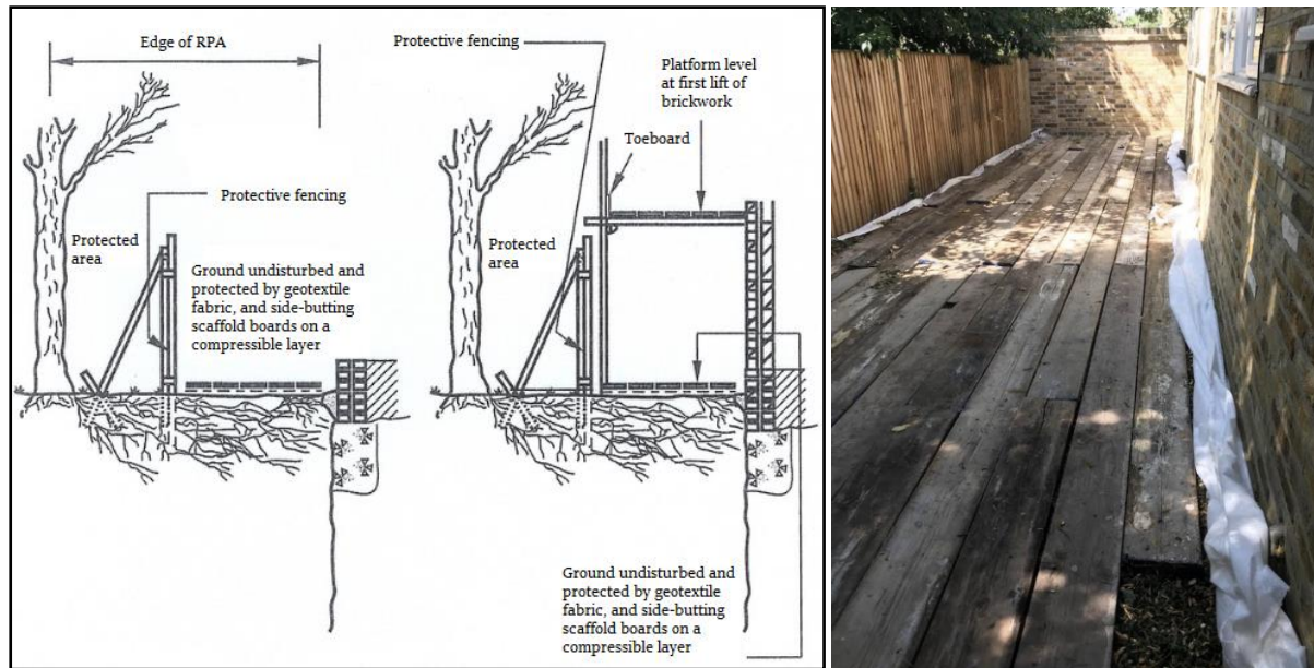
Figure 1: An example of ground protection on work areas within a RPA (BS 5837:2005).
