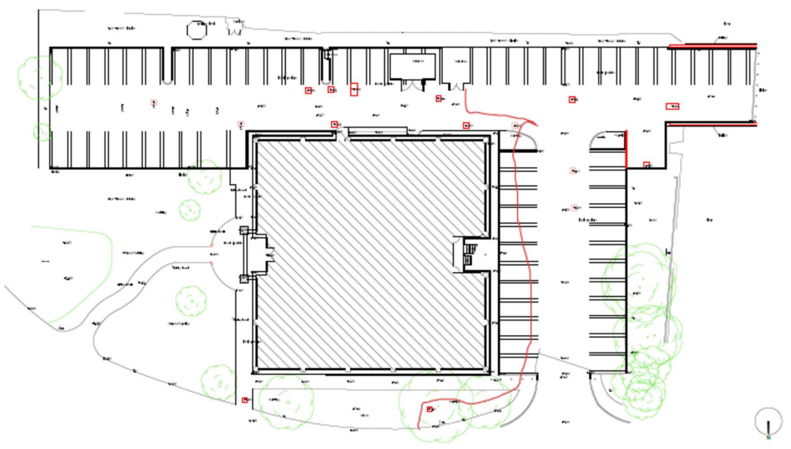
Figure 2.3 Proposed Site Plan of the Development.
