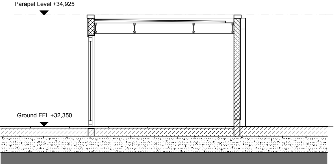
Bin Store Section AA
