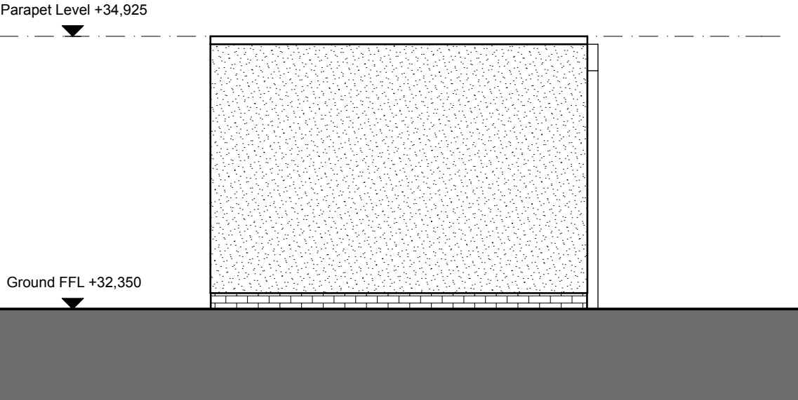
Bin Store Elevation 02
