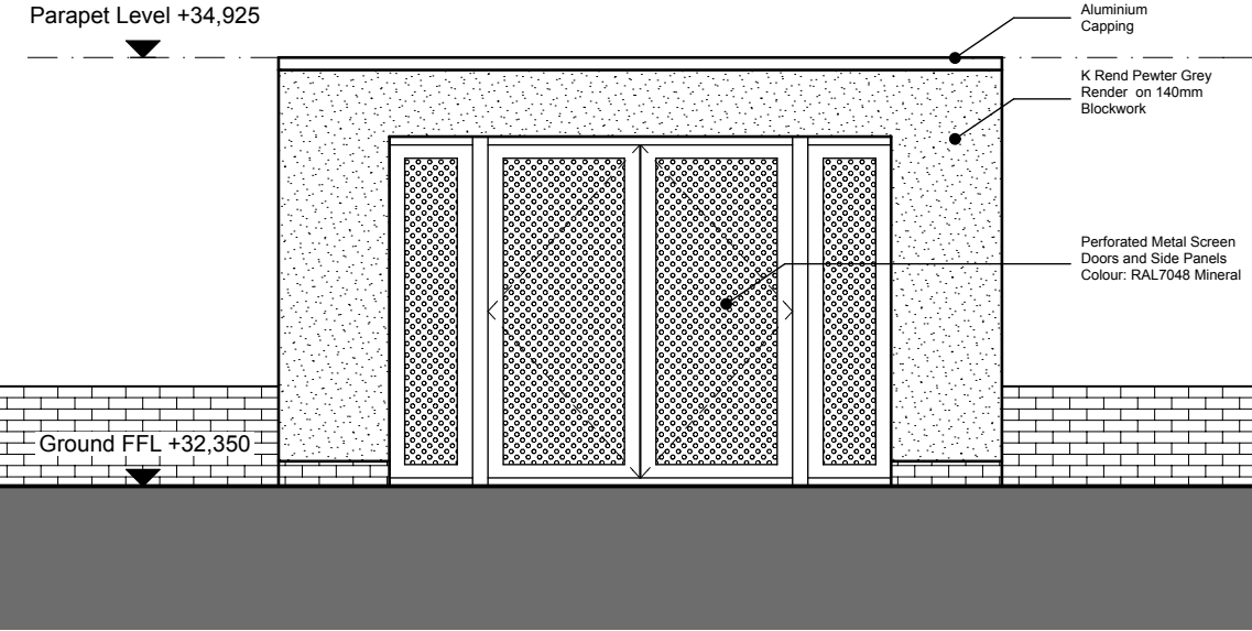
Bin Store Elevation 01
