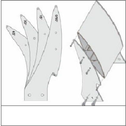
Horizontal Fin - Brise soleil Anodized aluminum Location: to curtain walling on south facades. Colour: Basalt grey, similar to RAL 7012
