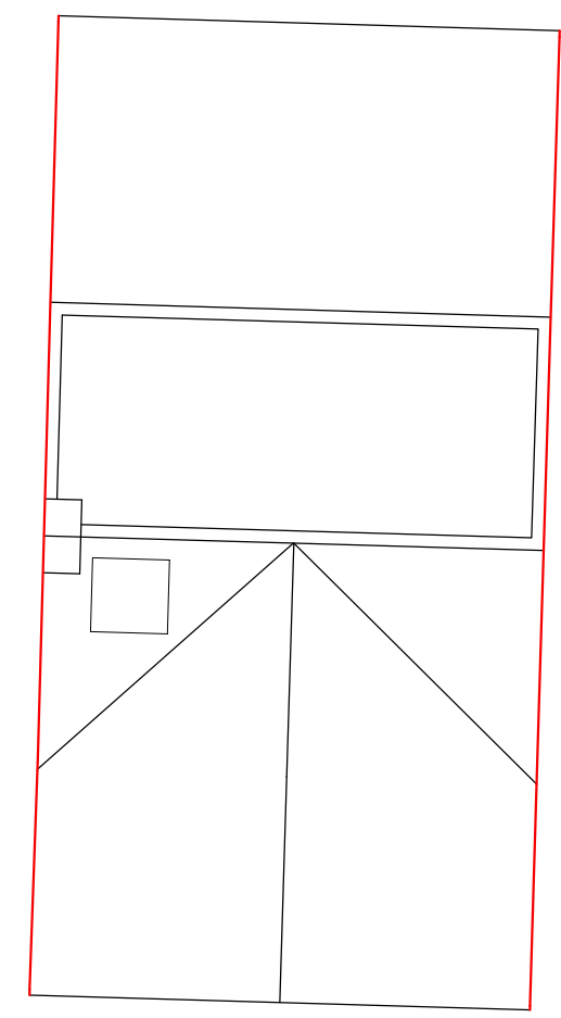
1:100 ROOF PLAN
