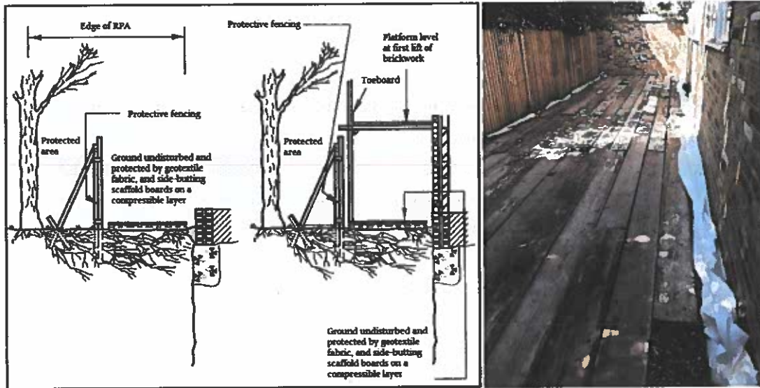
Photo 2. An example of heavy duty ground protection.
