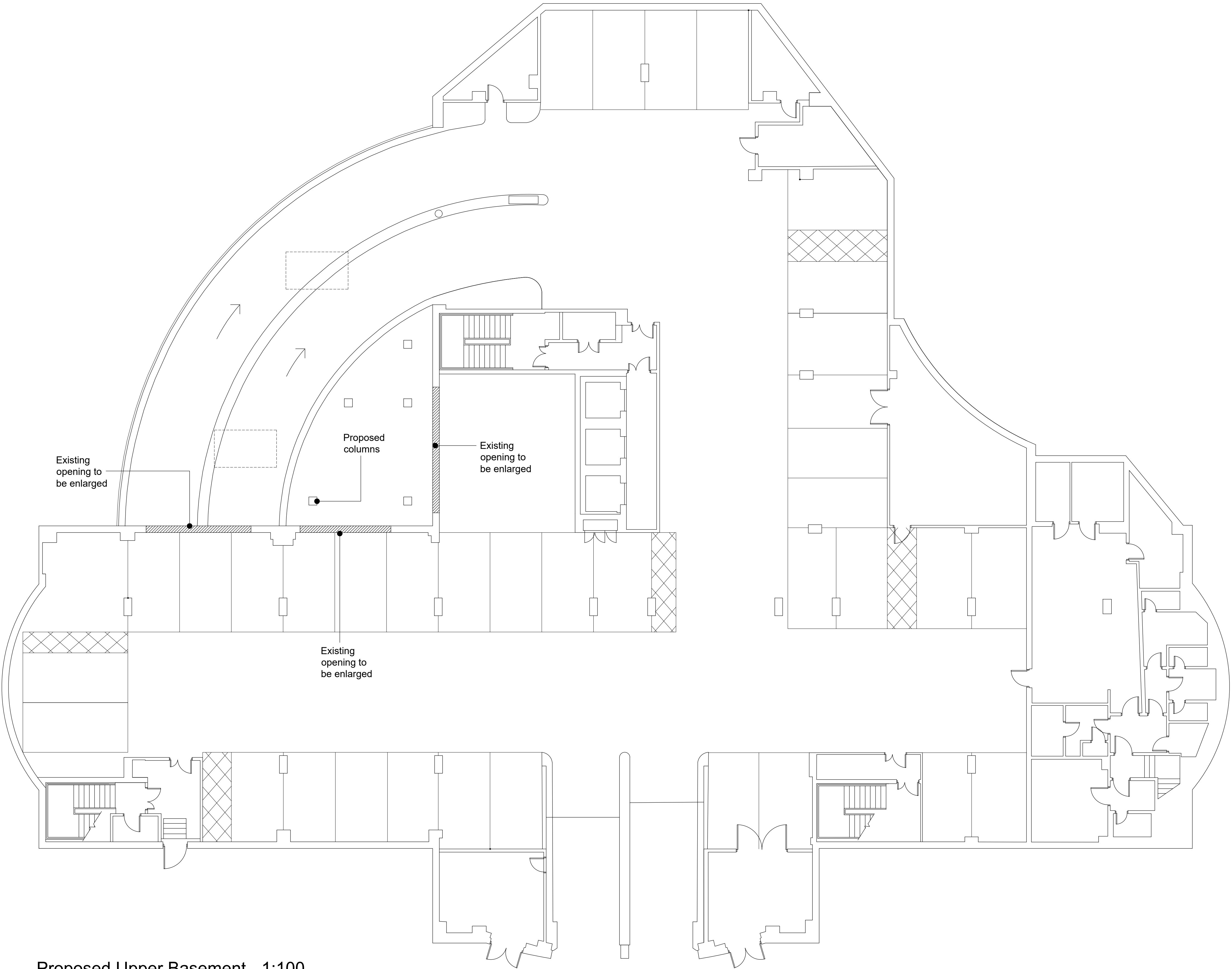
Proposed Upper Basement - 1:100
