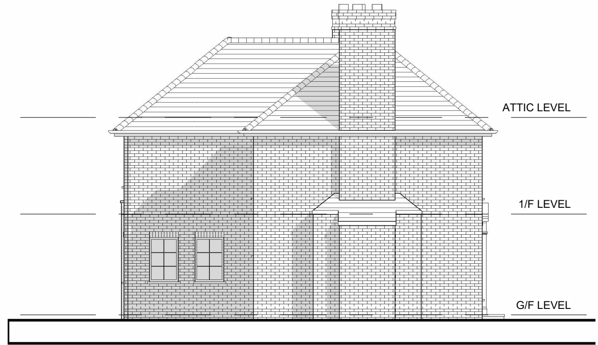
4 EXISTING WEST ELEVATION_
