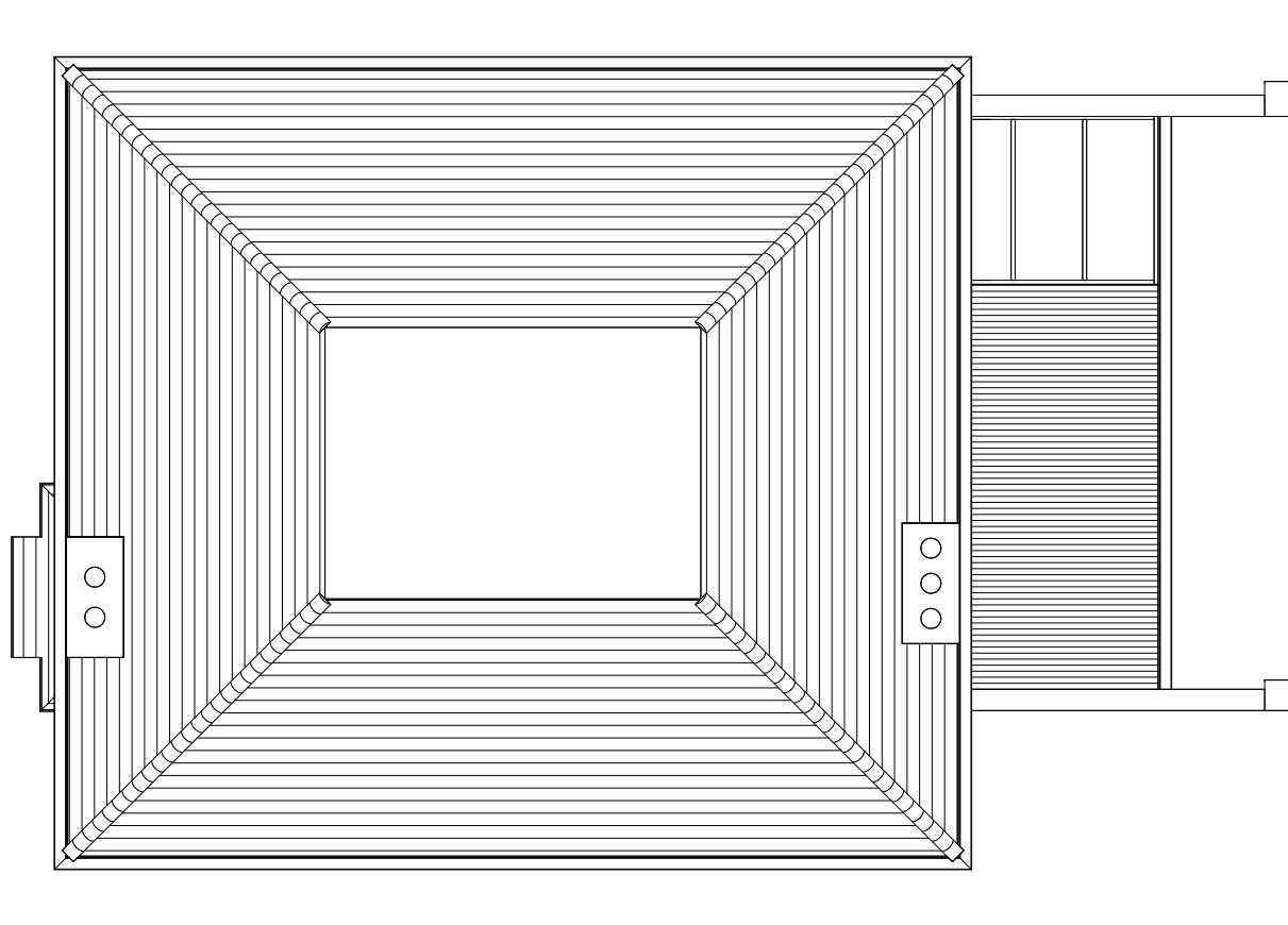
1 PROPOSED ROOF PLAN
