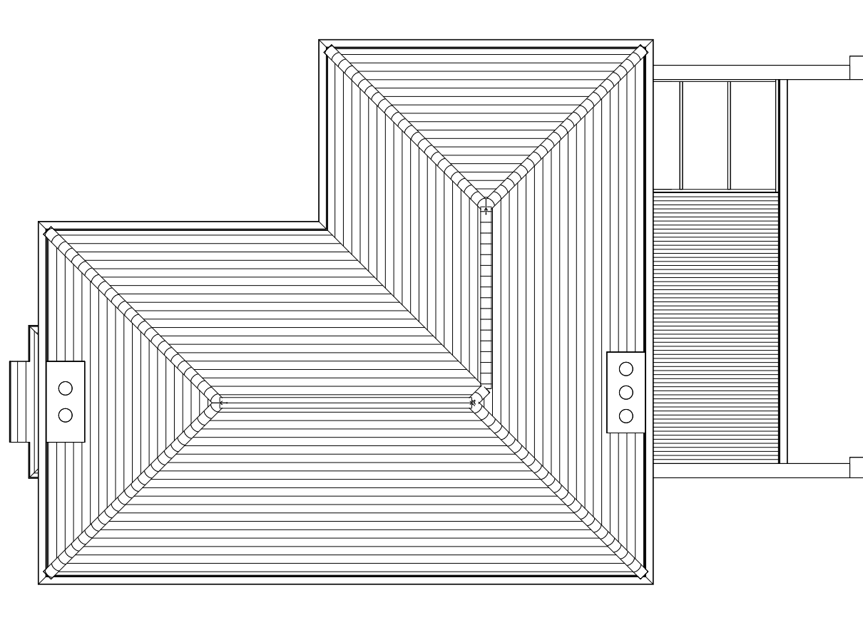
1 EXISTING ROOF PLAN
