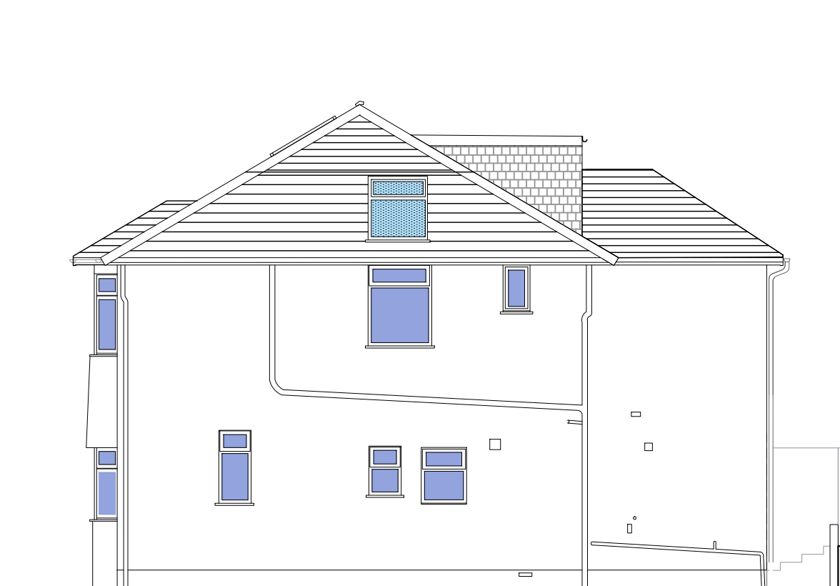
PROPOSED SIDE ELEVATION (WEST)
