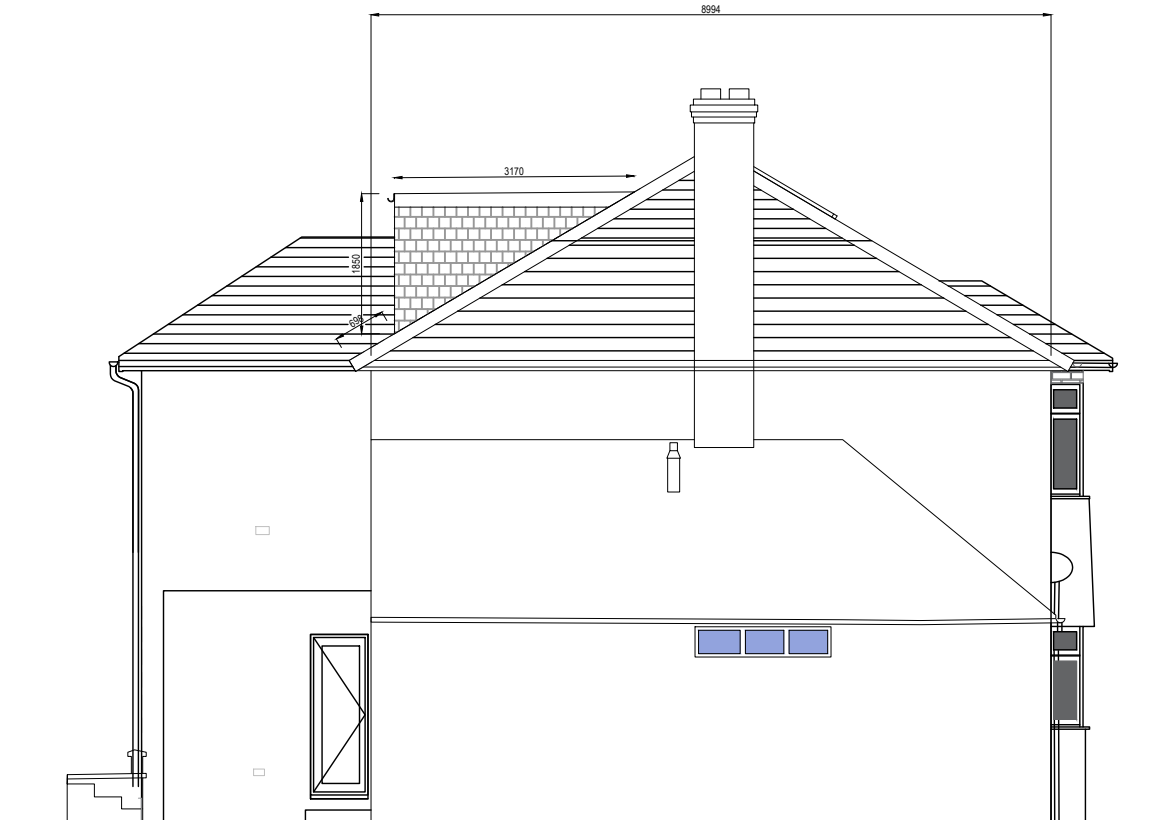
PROPOSED SIDE ELEVATION (EAST)
