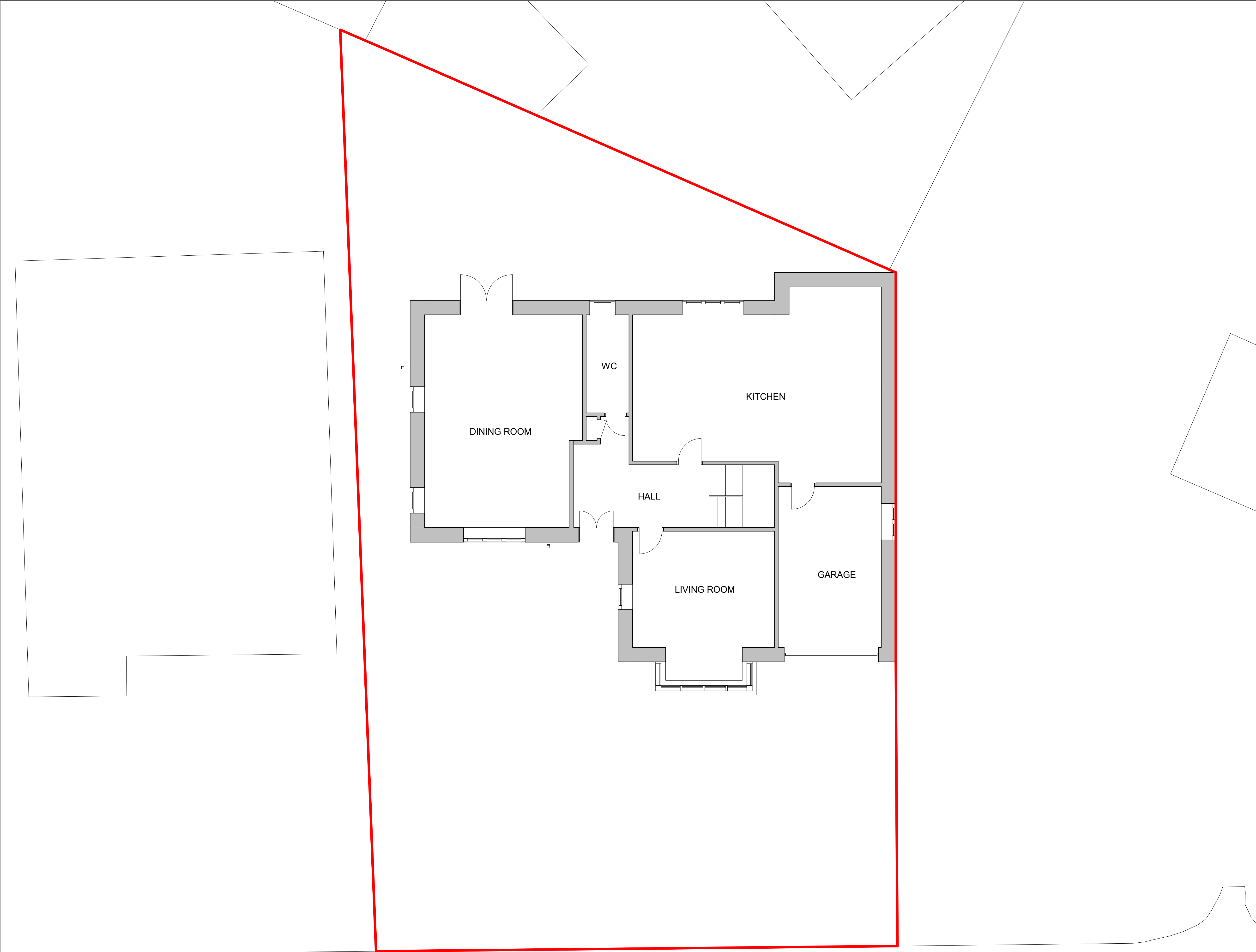
Ground Floor Existing 1 : 50
