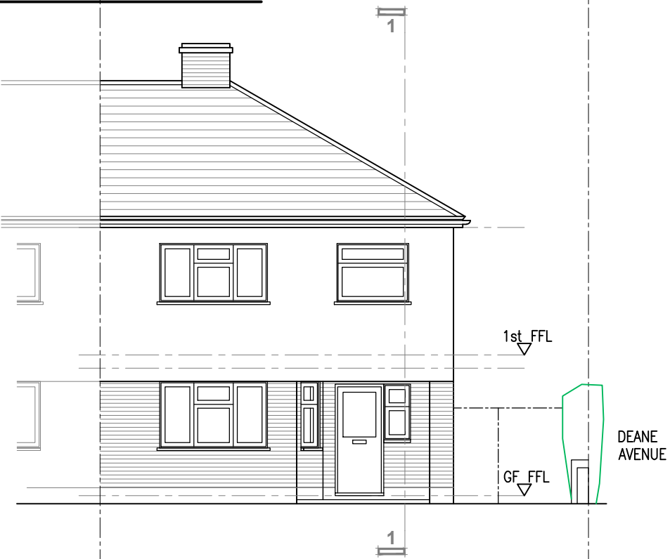
Front Elevation
