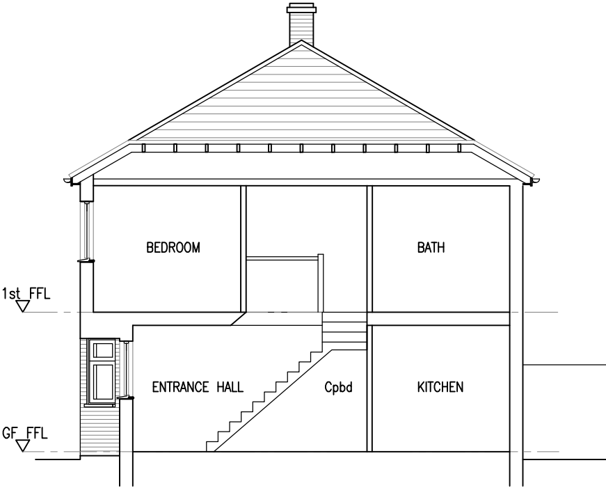
Section 1-1
