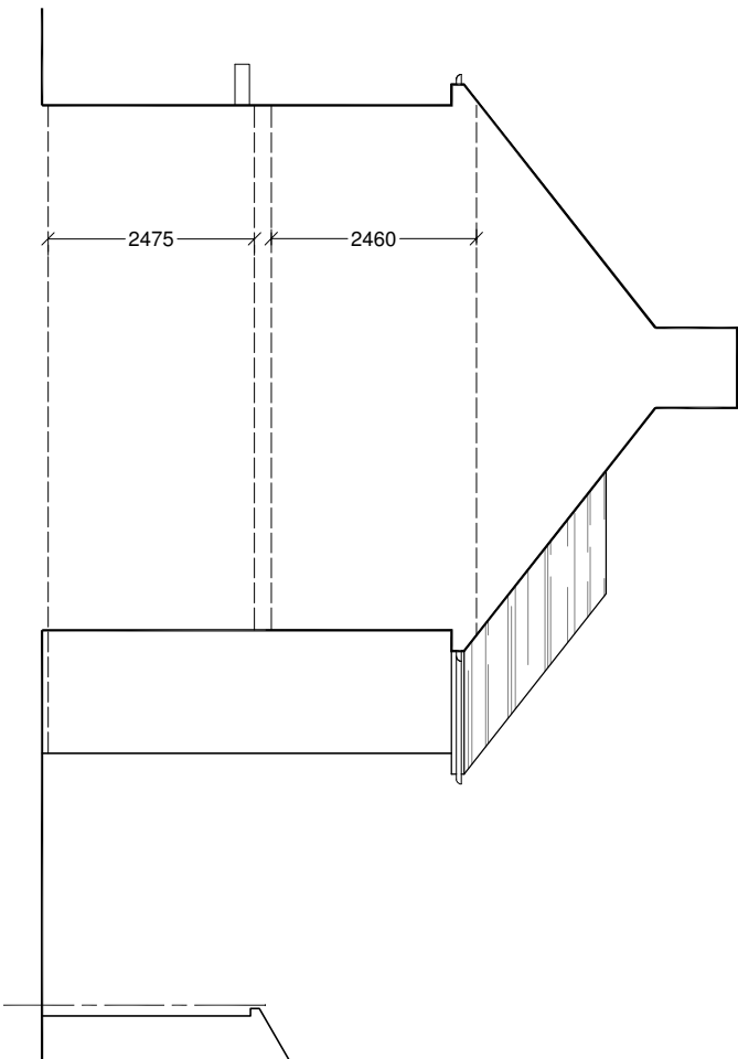
EAST ELEVATION
