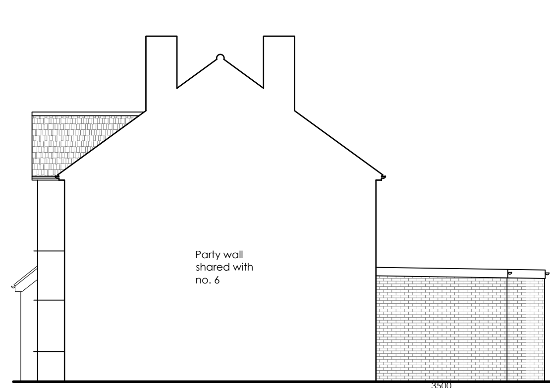
PROPOSED OPPOSITE SIDE ELEVATION
