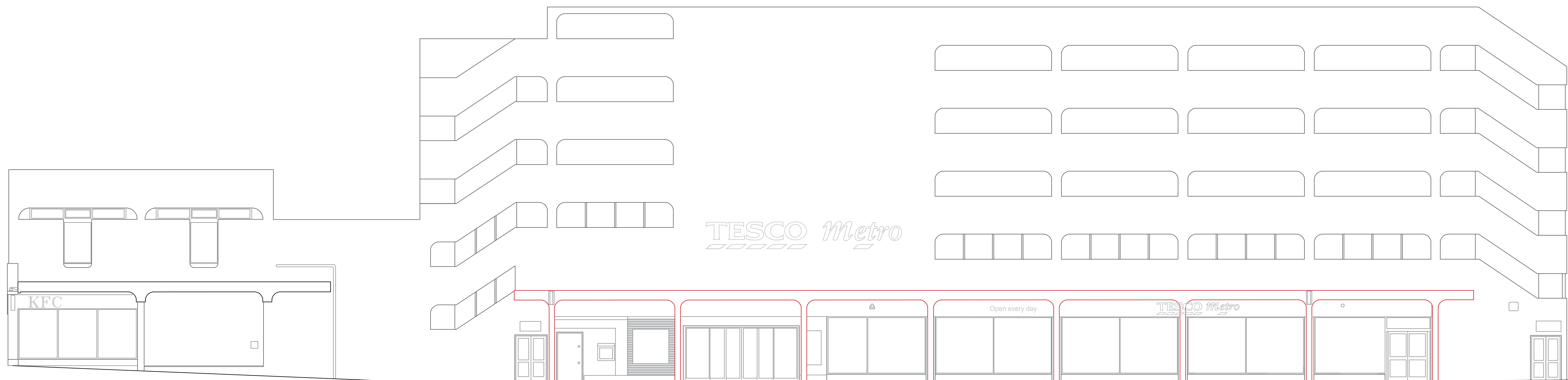
Existing Elevation
