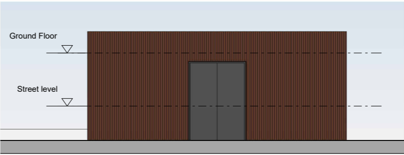
4 Elevation Refuse Storage - Front 1 : 100
