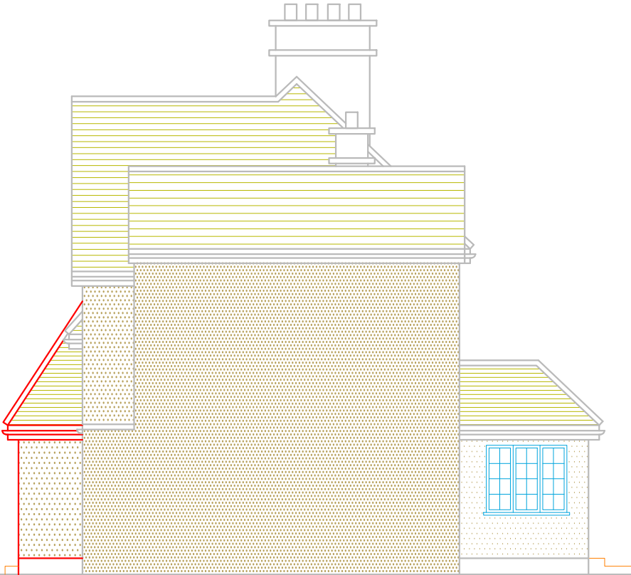
PROPOSED SIDE ELEVATION-1
