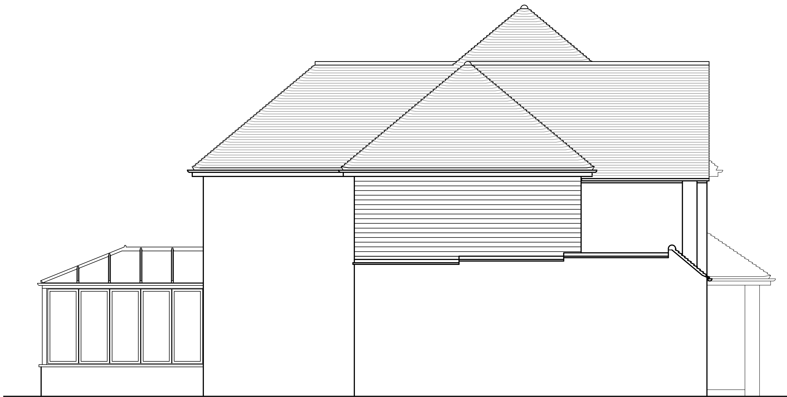
EXISTING SIDE (east) ELEVATION scale 1:50
