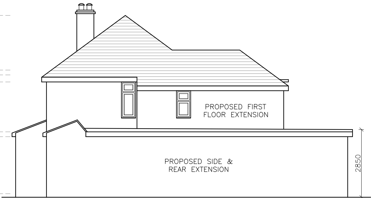
PROPOSED NORTH SIDE ELEVATION SCALE= 1:100
