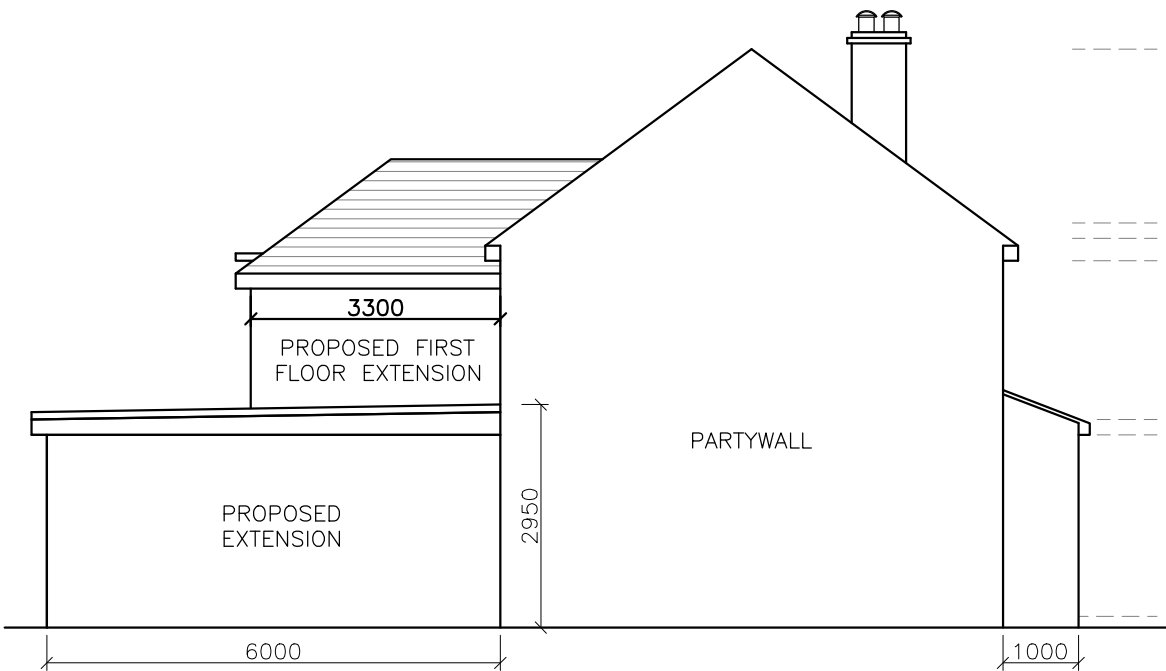
PROPOSED SOUTH SIDE ELEVATION SCALE= 1:100
