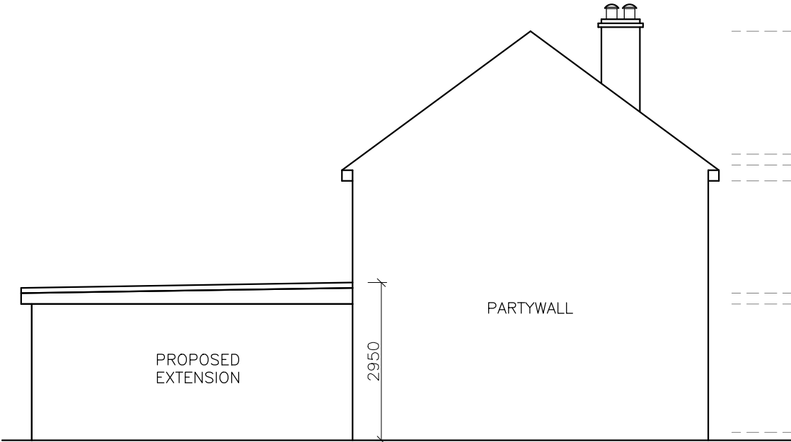
SCALE= 1:100 PROPOSED SOUTH SIDE ELEVATION
