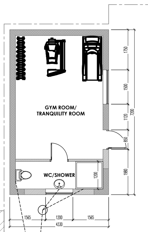
PROPOSED FLOOR PLAN SCALE 1/100
