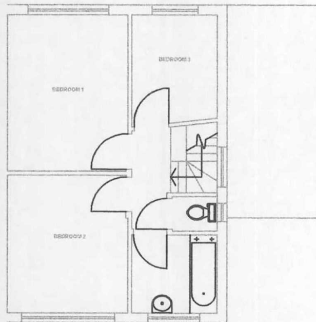
EXISTING 1ST FLOOR
