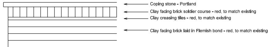
Parapet Detail to Rear Extension - 1:50
