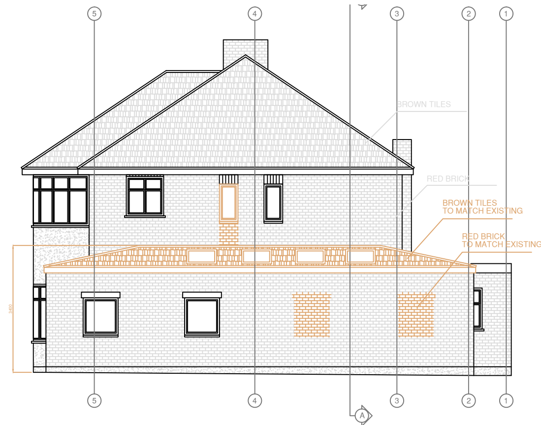
PROPOSED RIGHT SIDE ELEVATION
