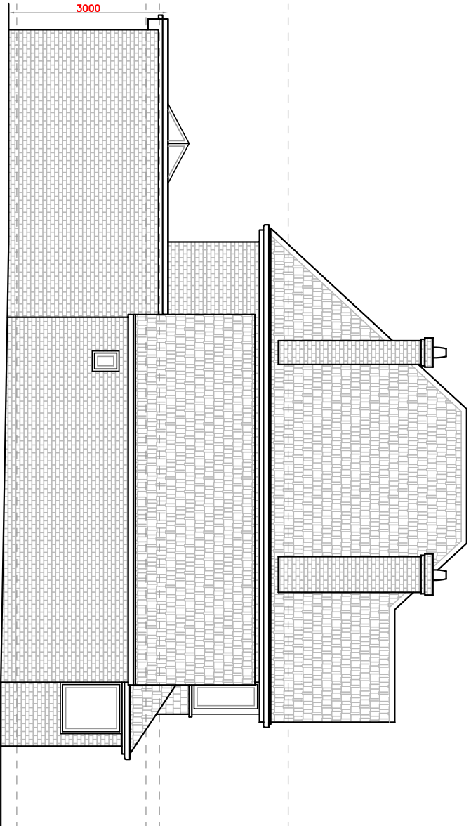
PROPOSED LEFT ELEVATION
