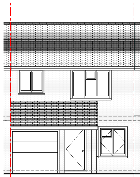
EIXISTING FRONT (1:100)
