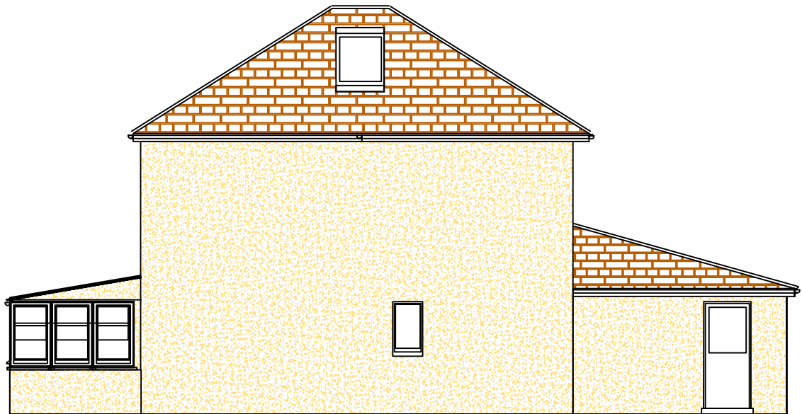
Proposed North Elevation (Facing 3 Larches)
