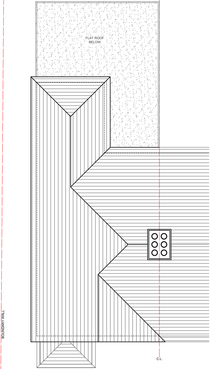
03- ROOF PLAN
