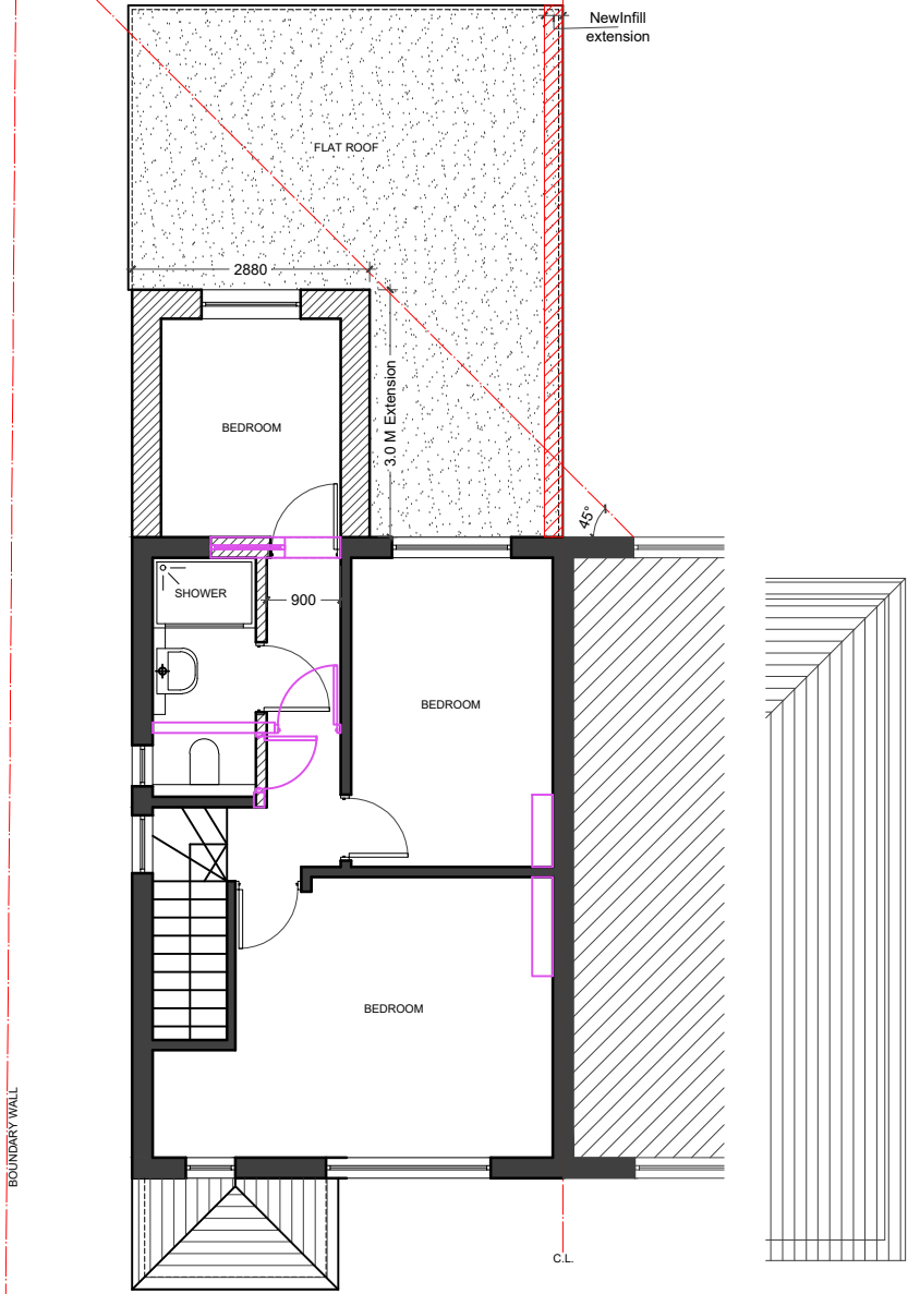
02- LOFT FLOOR PLAN
