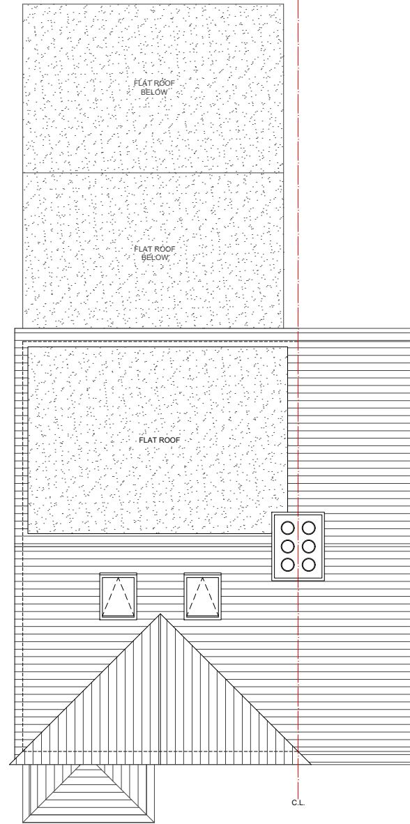
03- ROOF PLAN
