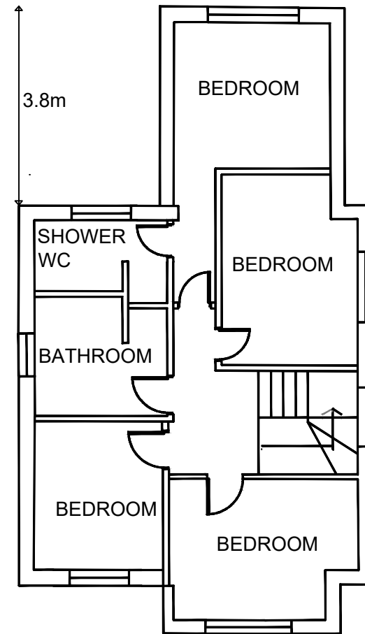
Existing 1st Floor Plan
