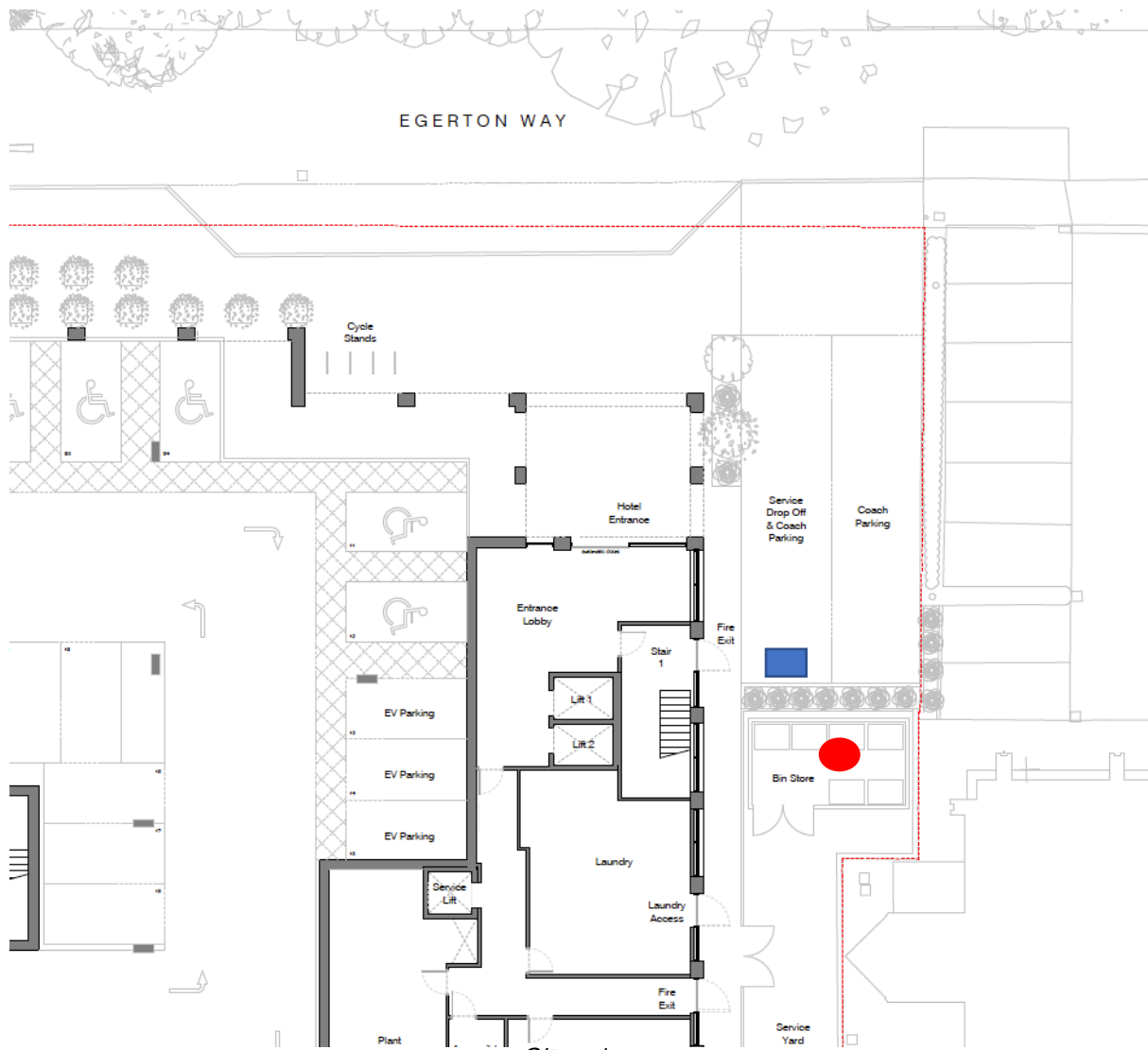
Site plan
