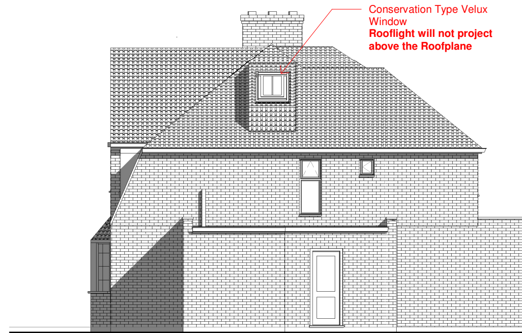
4 Proposed Side Elevation II. 1 : 100
