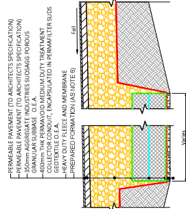
TYPICAL SECTION THROUGH PERMEABLE PAVEMENT AND PERMAVOID MEDIUM DUTY TREATMENT COLLECTOR CONDUIT
