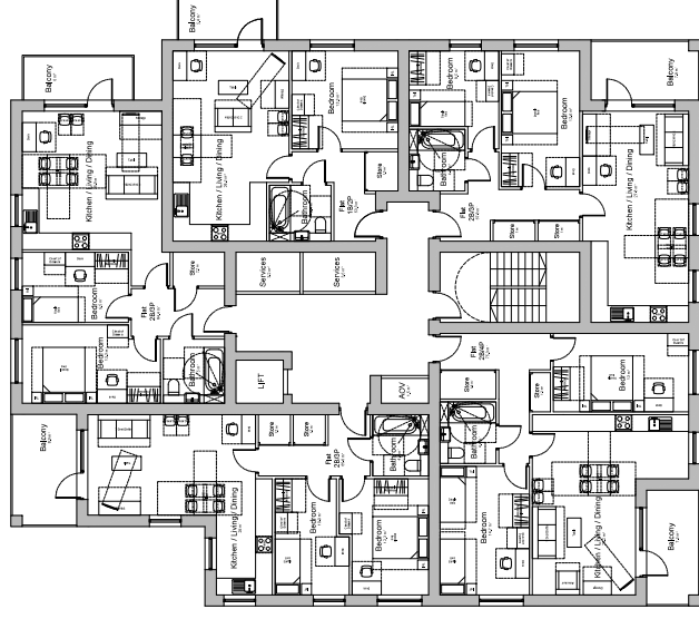
Proposed First /Second Floor Plan
