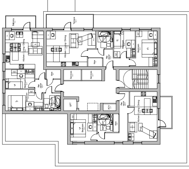
Proposed Third Floor Plan
