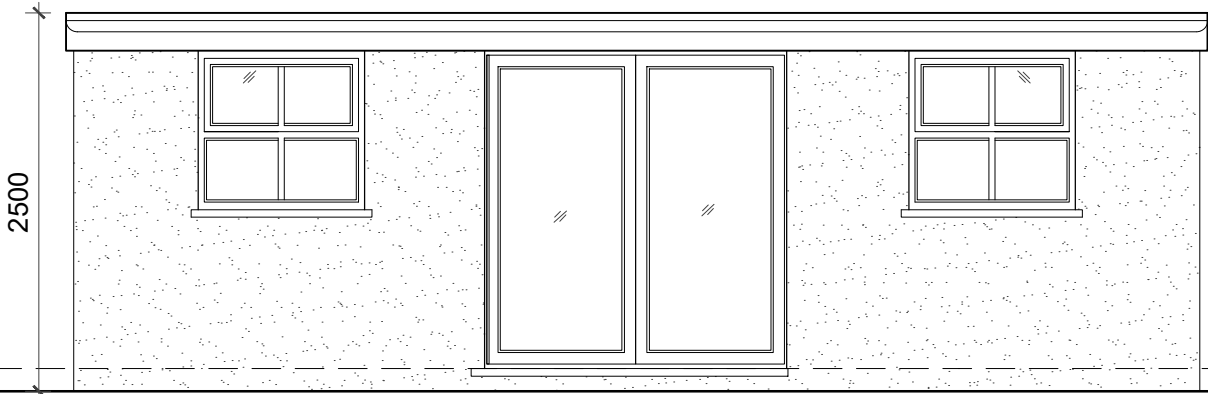
03- FRONT ELEVATION
