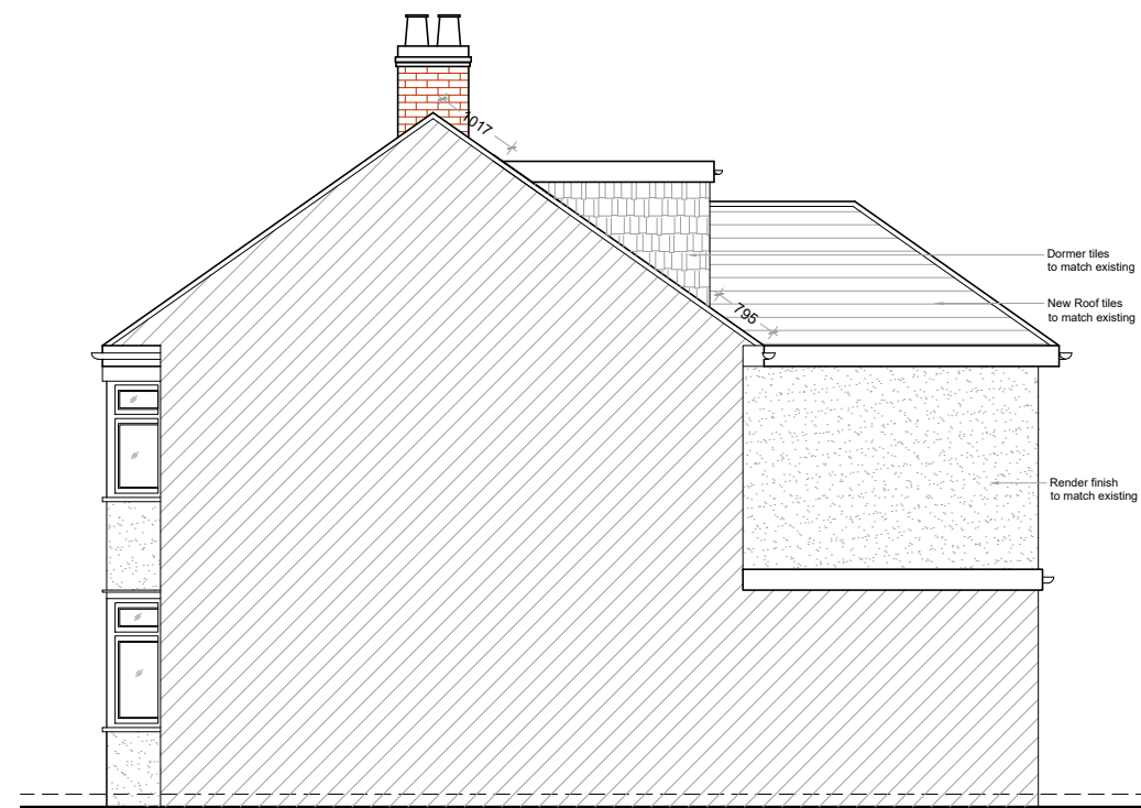
04 - RIGHT SIDE ELEVATION
