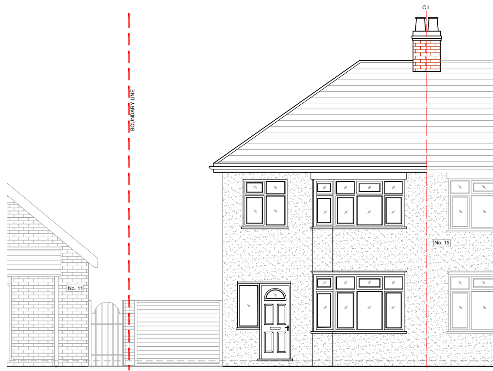
04 - FRONT ELEVATION
