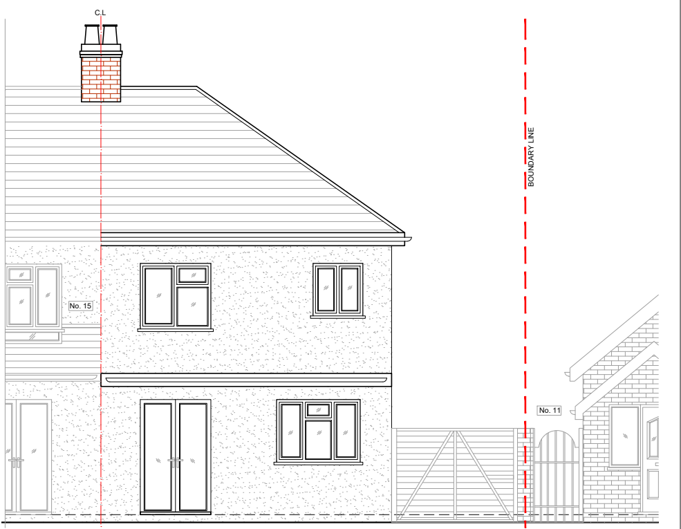
06 - REAR ELEVATION
