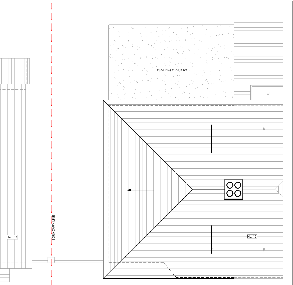
03 - ROOF PLAN
