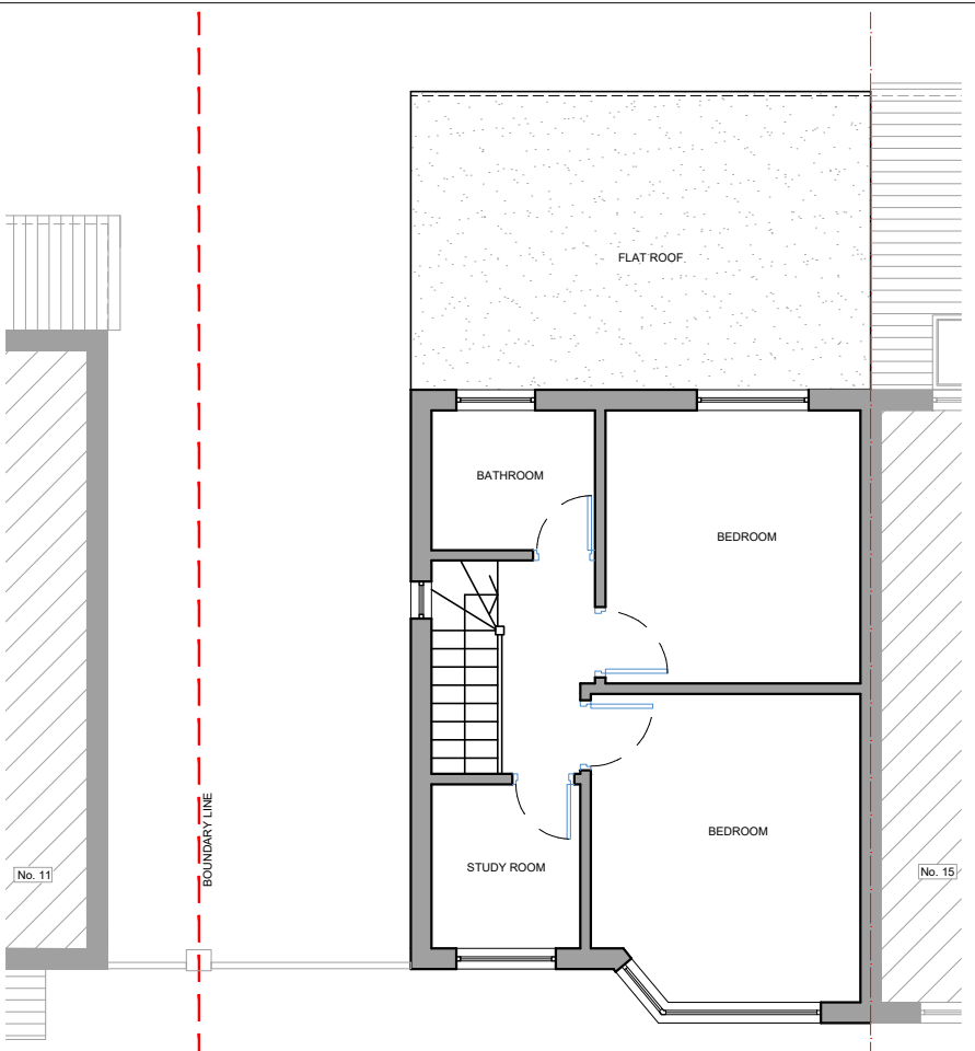
02 - FIRST FLOOR PLAN
