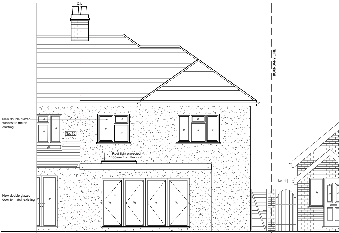
02 - REAR ELEVATION
