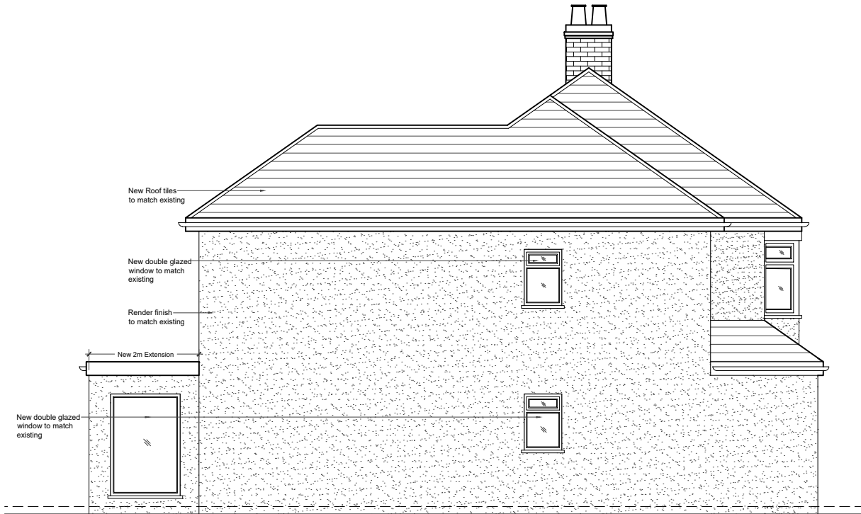
03 - SIDE ELEVATION (LEFT SIDE)
