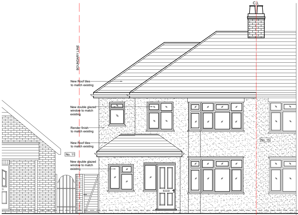
01 - FRONT ELEVATION
