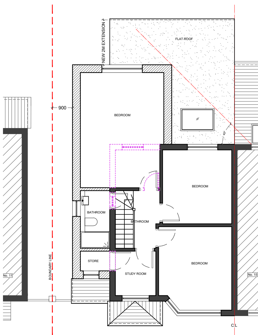
02 - FIRST FLOOR PLAN
