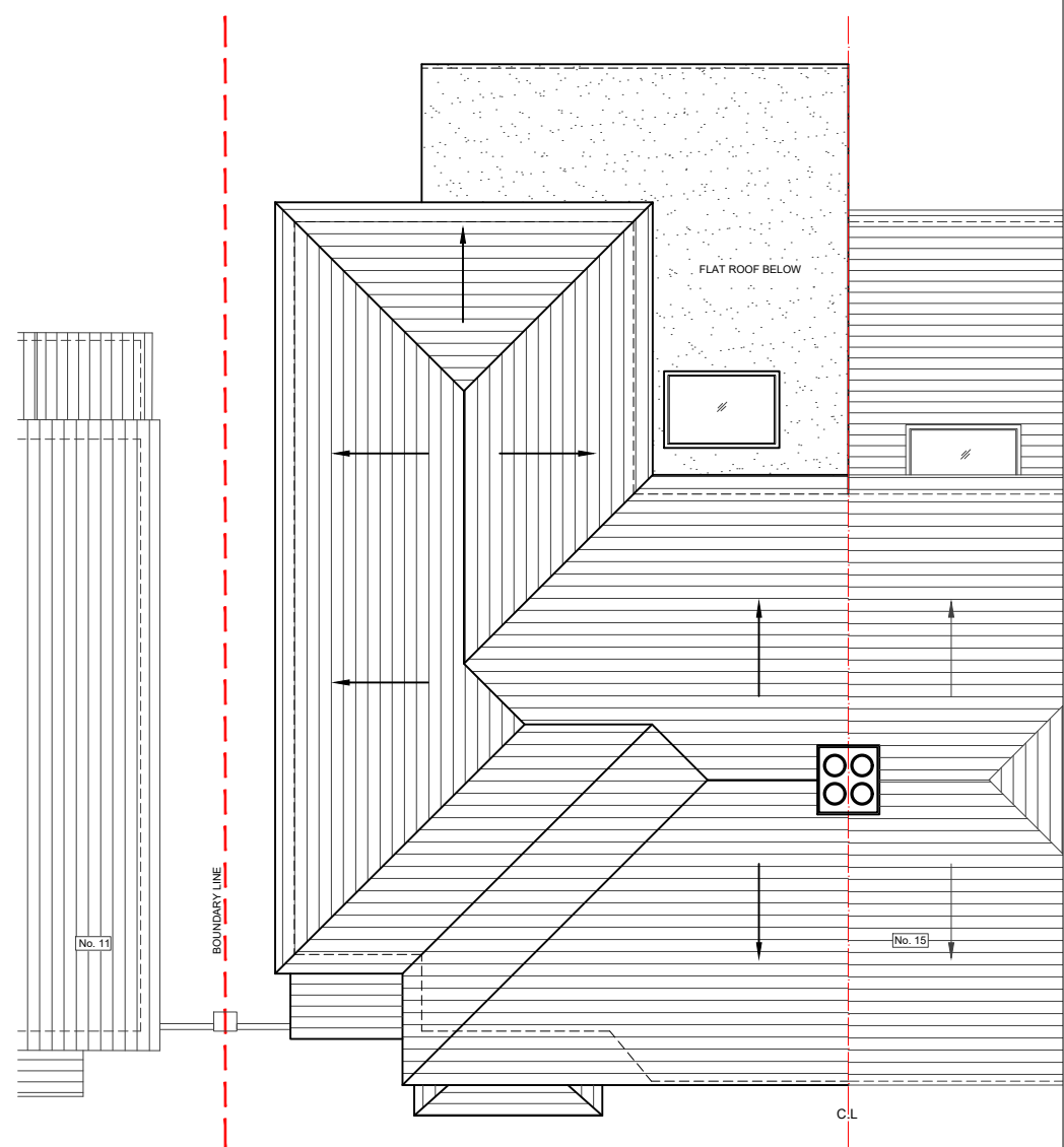
03 - ROOF PLAN
